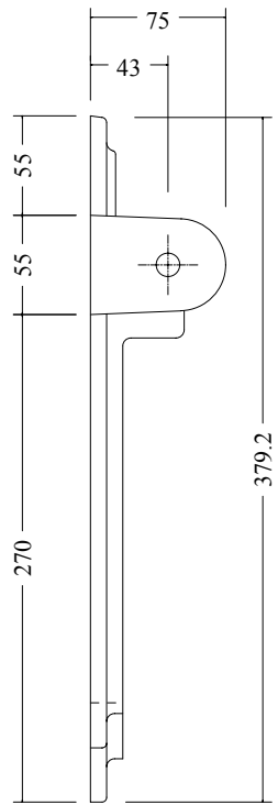
SIDE ELEVATION
